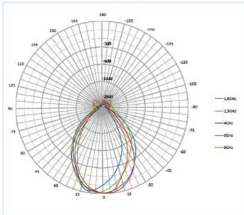
HyperLOG Horizontal Pattern
