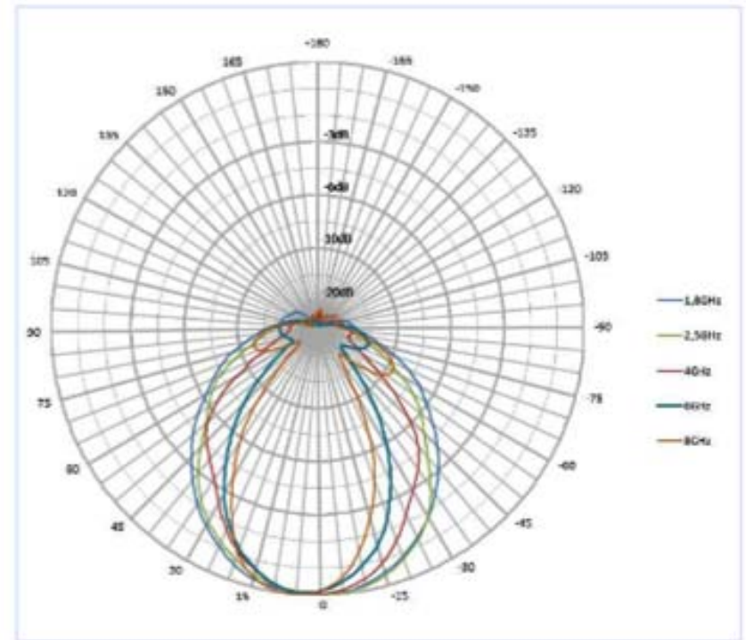
HyperLOG Vertical Pattern
